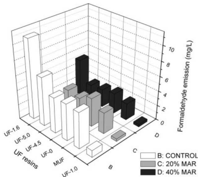
Figure 2 Effects of the addition of MAR powder on the formaldehyde emissions of hardwood plywood fabricated with UF resins.
