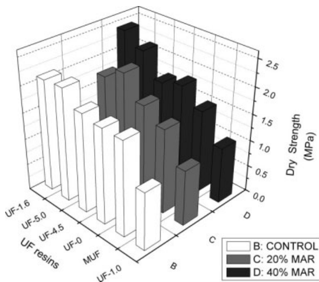
Figure 1 Effects of the addition of MAR powder on the bonding strength of hardwood plywood fabricated with UF resins.
