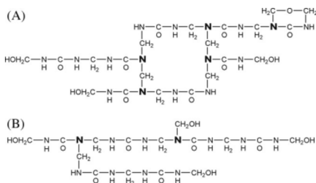
Figure 3 Models for ethanol-insoluble fractions of (A) UF-1.0 and (B) UF-5.0. N (in bold) indicates tertiary nitrogen; N (not in bold) indicates secondary nitrogen.
